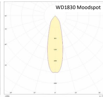
Polar chart 25° optic
