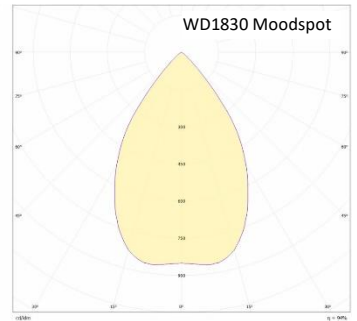
Polar chart 60° optic
