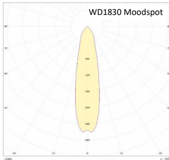
Polar chart 15° optic
