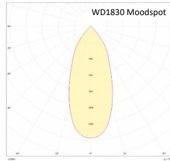
Polar chart 40° optic
